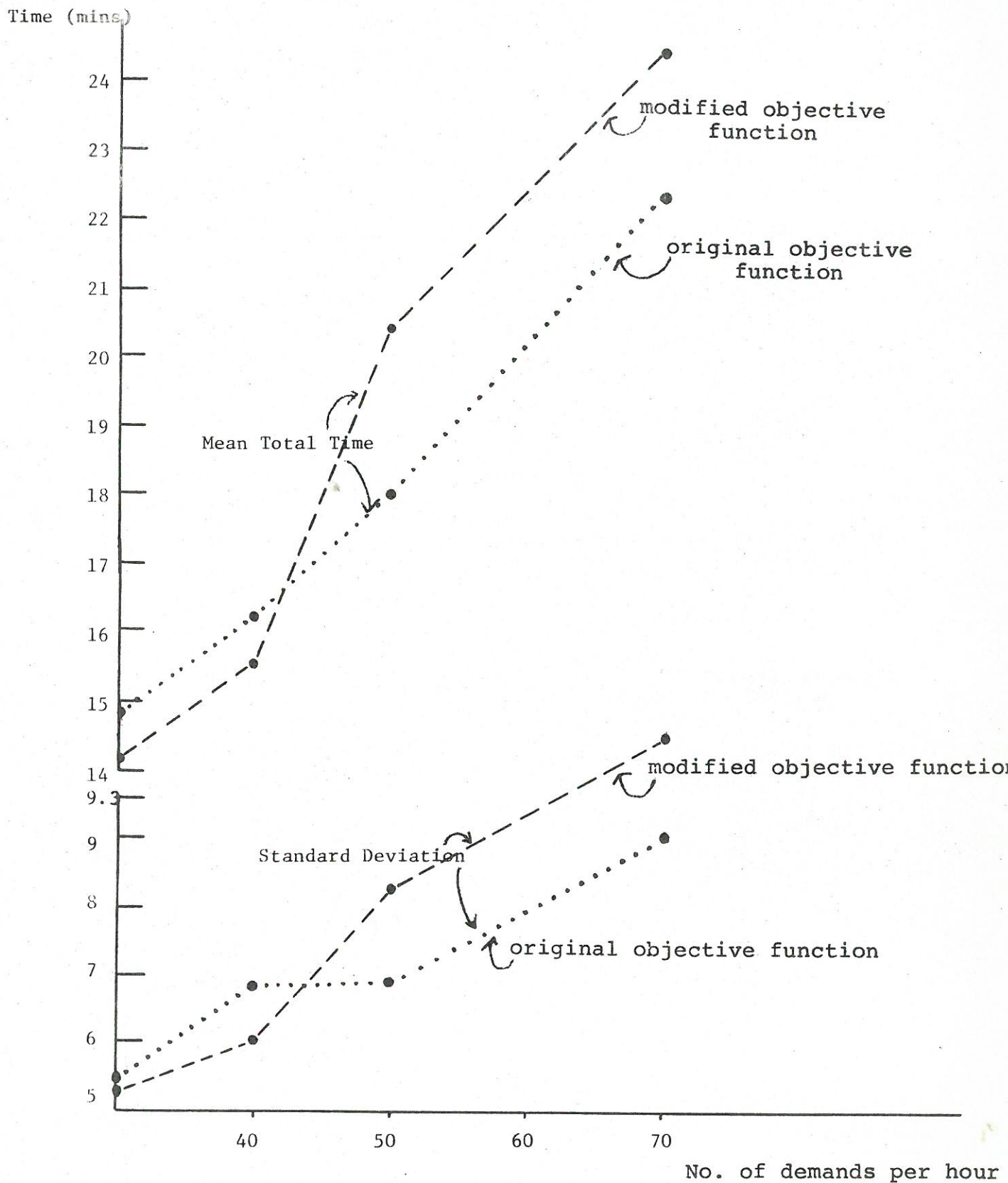
FIGURE B-1: PERFORMANCE UNDER VARYING LOADS
